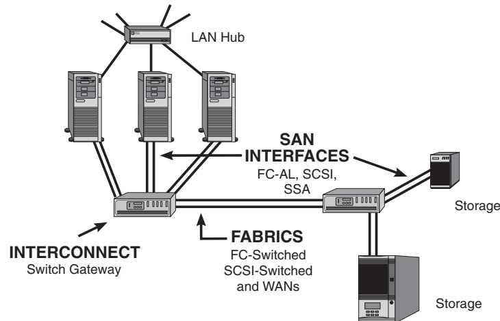
Figure 1.2 SAN network terminology.
